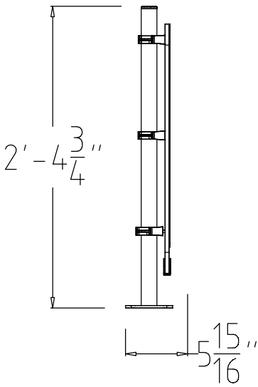
FRONT ELEVATION
