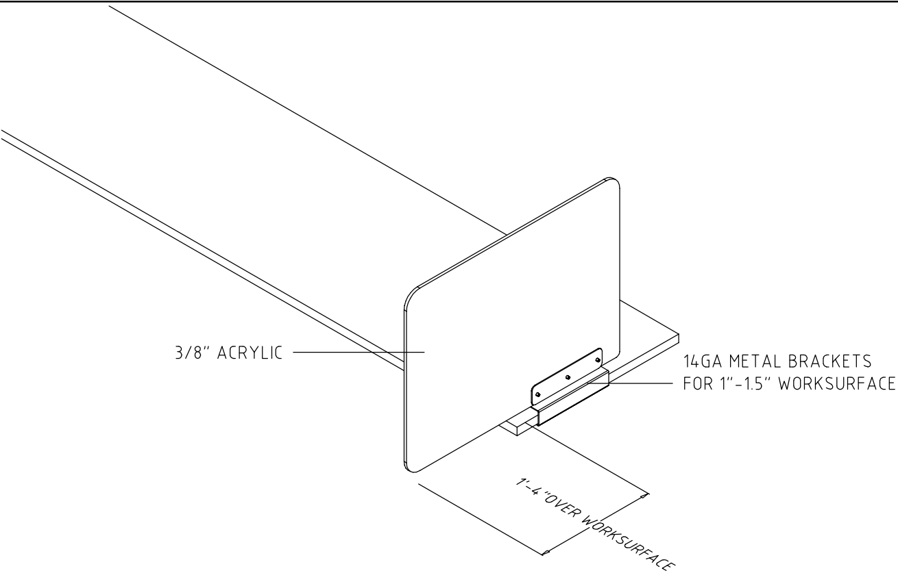
ISOMETRIC VIEW
